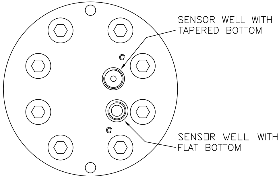
TOP VIEW JVx-60xG
