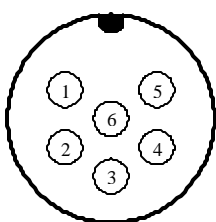
Pinout looking at male connector on sensor
